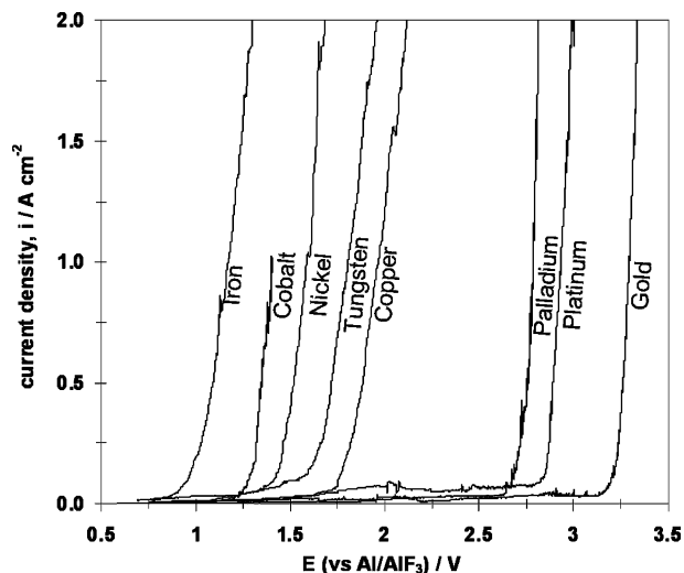
Fig. 3. Steady state current versus potential ( 0.002 \text{ V s}^{-1} ) curves on metal electrodes in oxide-free cryolite melt [CR = 2.2; 5%wt. \text{CaF}_2 ; T = 1273 \text{ K} ].
